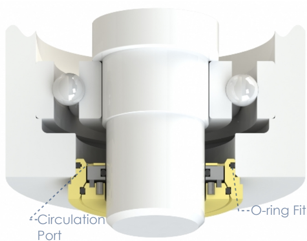
Magnum-P V6S
